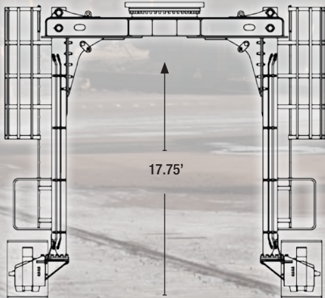
HI-TOP/LOCOMOTIVE CLEARANCE
